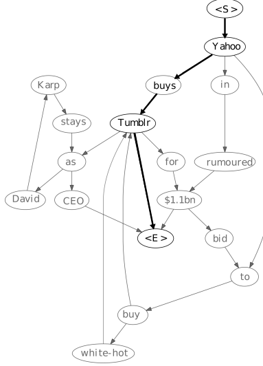
Fig. 1: Word graph constructed from the sentences: "Yahoo in rumoured $1.1bn bid to buy white-hot Tumblr", "Yahoo buys Tumblr as David Karp stays as CEO", "Yahoo to buy Tumblr for $1.1bn". The shortest path is highlighted.
