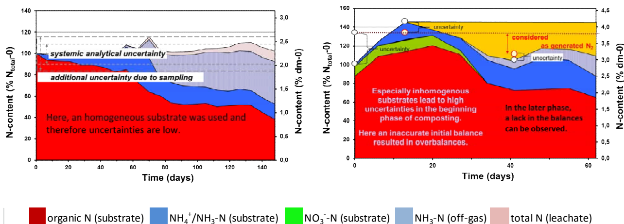
Figure 2. N-balance-series of composting processes: Left) Balance with high accuracy; Right) Balance with lower accuracy and a lack due to compounds not measured quantitatively (dm -0: initial dry-matter content)
