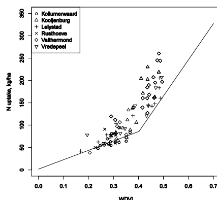
Figure 1. Relationship between WDI and N uptake in potato. See main text for further explanation.
