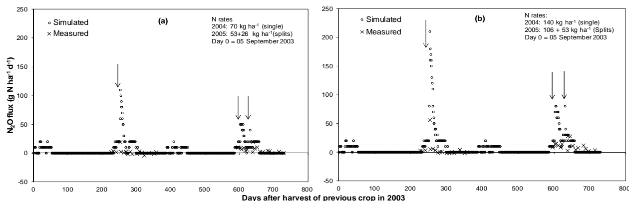
Figure 1. Measured and simulated \text{N}_2\text{O} fluxes as influenced by N fertilizer rates applied (arrows) to spring barley.
