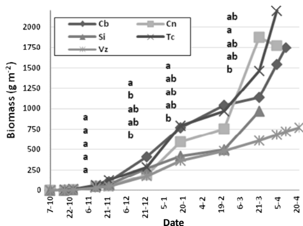
Figure 2. Biomass evolution (g m -2 ). Cb: Barley, Cn: Rye, Si: Mustard, Tc: Triticale, Vz: Vetch.
