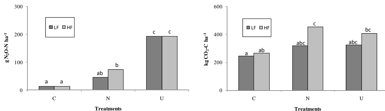
Figure 1. Cumulative \text{N}_2\text{O} and \text{CO}_2 emissions during the experimental period.
