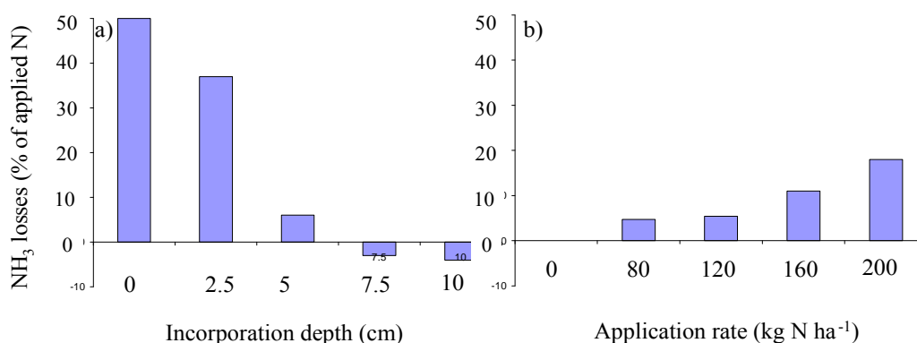
Figure 1. Cumulative \text{NH}_3 losses following banding urea in response to a) incorporation depth and b) application rate.
