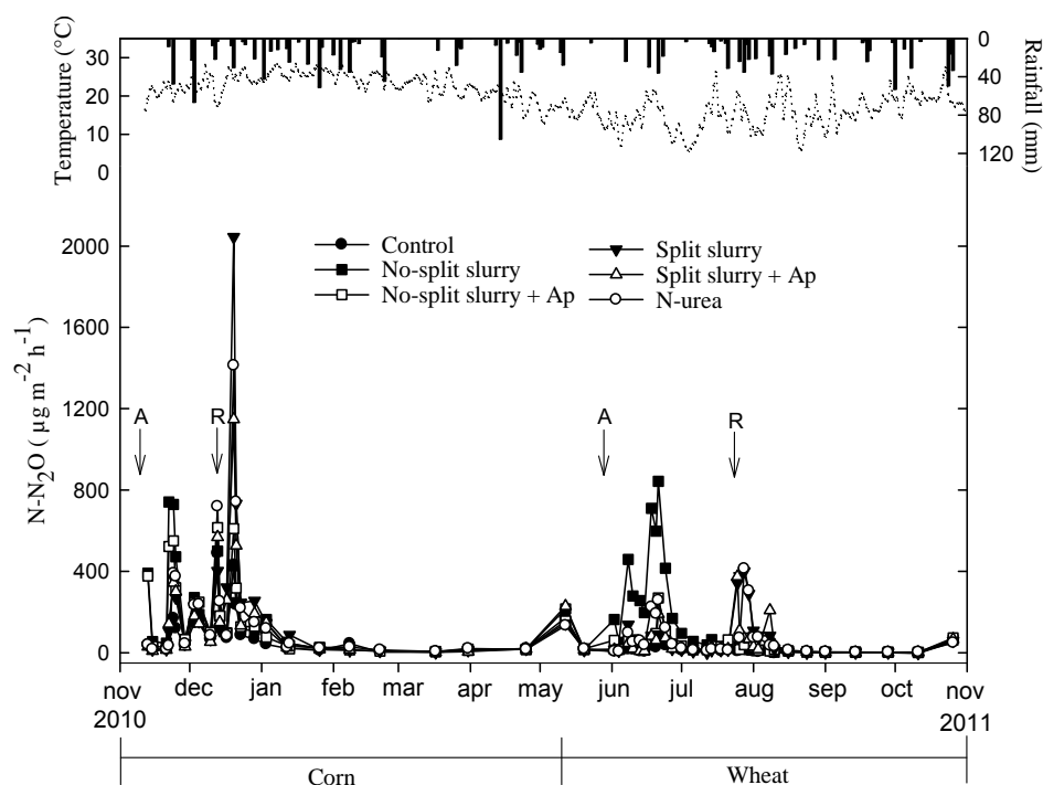
Figure 1. Temporal variation of rainfall and temperature and soil-surface \text{N}_2\text{O} flux from a soil cropped to no-till corn and wheat amended with N-urea, non-split and split pig slurry, with and without nitrification inhibitor. Ap=Agrotain plus, containing 81% of dicyandiamide (DCD); A=Application of pig slurry; R=Reapplication of pig slurry.
