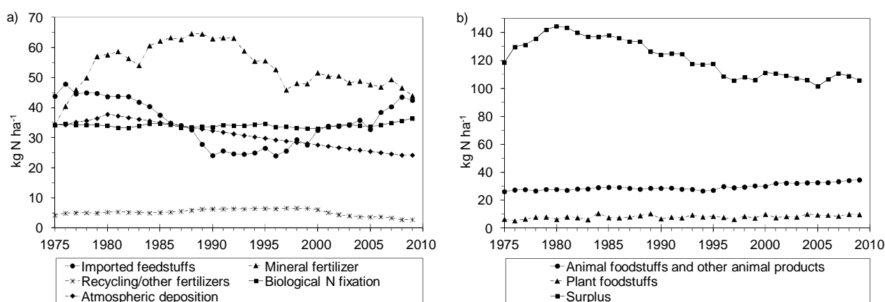
Figure 1. Development of N amounts in balance items of Swiss agriculture from 1975 to 2009 (in \text{kg N ha}^{-1} UAA). a) Input items. b) Output items and surplus.
