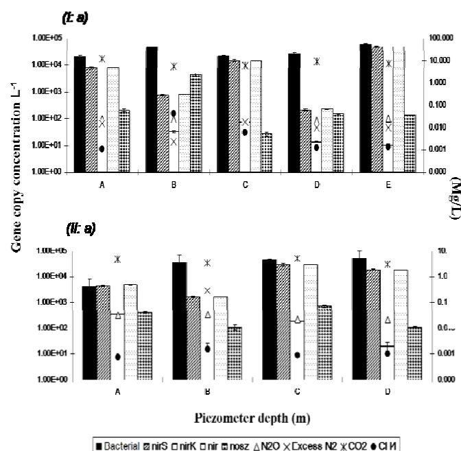
Figure 1. Mean groundwater nirK , nirS , nosZ and bacterial 16S rRNA GCC L^{-1} filtered at (OP I: a) spring barley, (Depth – A & B=5 m) (Depth – C & D=10 m); (Depth – E=20 m) (II: a) DG grazed clover ryegrass grassland.
