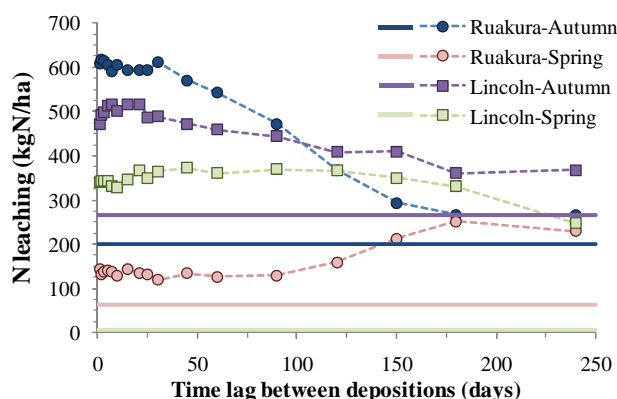
Figure 1. N leaching under overlapping urine depositions simulated in two locations and months. Data is average for all years of simulations with 500 kg N ha -1 depositions, with irrigation, and high fertiliser. Solid lines represent a single 500 kg N ha -1 urine patch.
