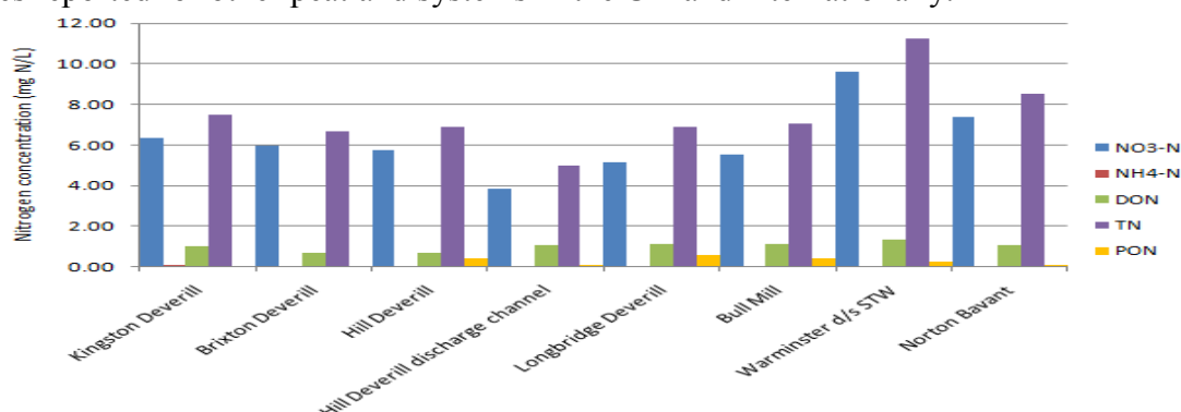
Figure 1. Nitrogen species concentration in the River Wylfe
