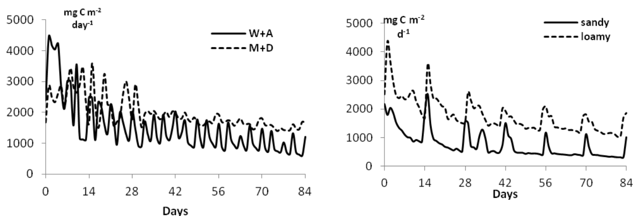
Figure 3a,b: C-CO 2 emission during decomposition of wheat+alfalfa mulch (W+A) and maize+dolichos mulch (M+D) on loamy soil (left) and comparison of sandy and loamy soil with decomposing M+D mulch (right). Peaks correspond to application of rain on columns.
