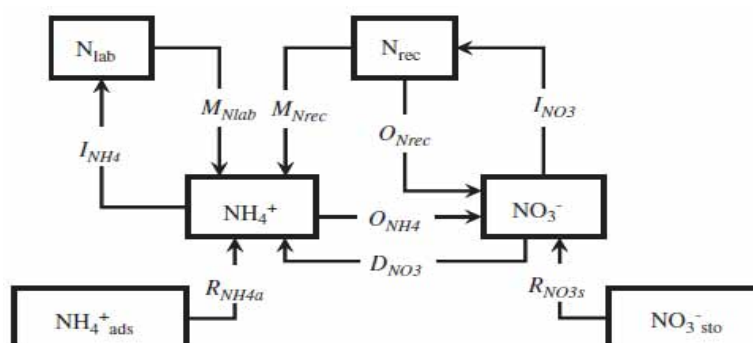
Figure 1. 15 N tracing model (Müller et al., 2007) (N lab = labile soil organic N, N rec = recalcitrant soil organic N, NH 4 + ads = adsorbed NH 4 + , NO 3 - sto = stored NO 3 - , M Nlab = mineralisation of N lab , M Nrec = mineralisation of N rec , I NH4 = immobilisation of NH 4 + , I NO3 = immobilisation of NO 3 - , O Nrec = oxidation of N rec to NO 3 - , O NH4 = oxidation of NH 4 + to NO 3 - , D NO3 = dissimilatory reduction of NO 3 - to NH 4 + , R NH4a = release of adsorbed NH 4 + , and R NO3s = release of stored NO 3 - ).
