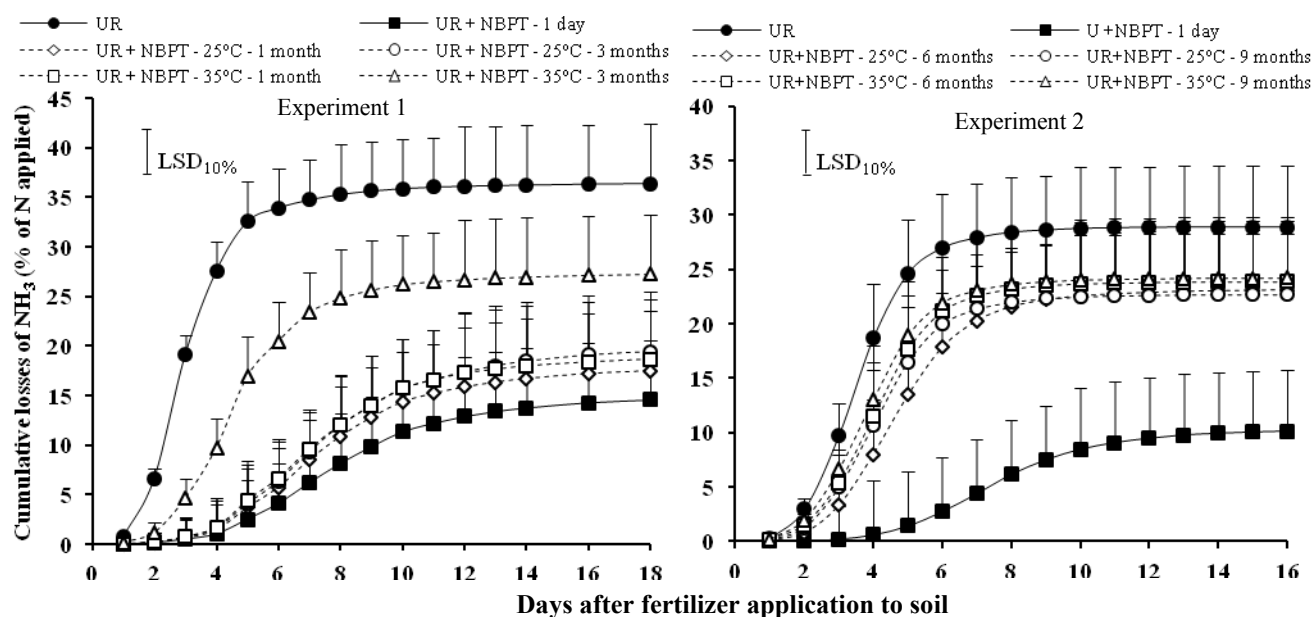
Figure 1. Cumulative losses of \text{NH}_3 after surface application of urea (UR) with or without the urease inhibitor (NBPT) stored at different temperatures and time periods. Data with overlapping vertical bars do not differ (Tukey, p \leq 0.10 ).
