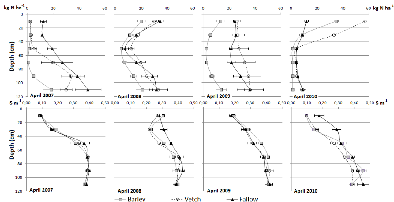
Figure 2. Distribution of soil \text{Nmin} ( \text{kg N ha}^{-1} ) and saturated paste extract soil electrical conductivity ( \text{S m}^{-1} ) by depth at the end of the cover crop growing season (maize sowing), as influenced by the cover crop treatment.
