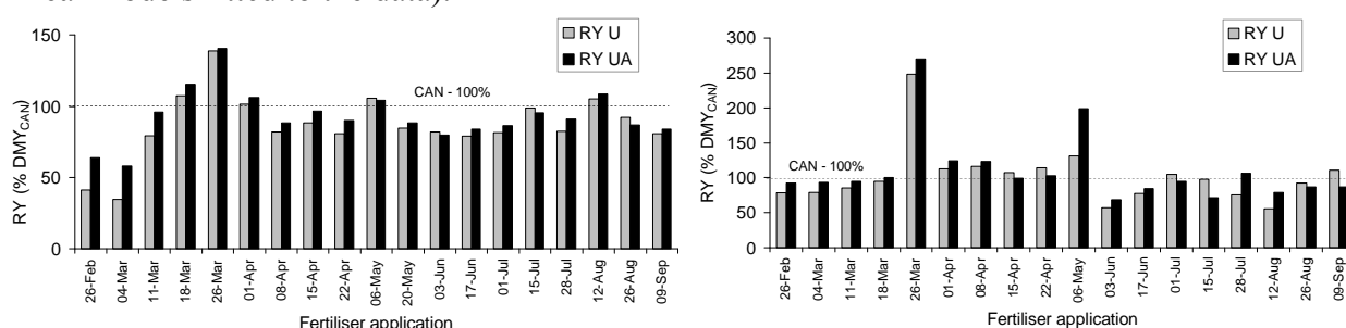
Figure 1. DMV of U and UA relative to CAN four weeks (left) and during the period between four and eight weeks (right) after fertiliser application.
