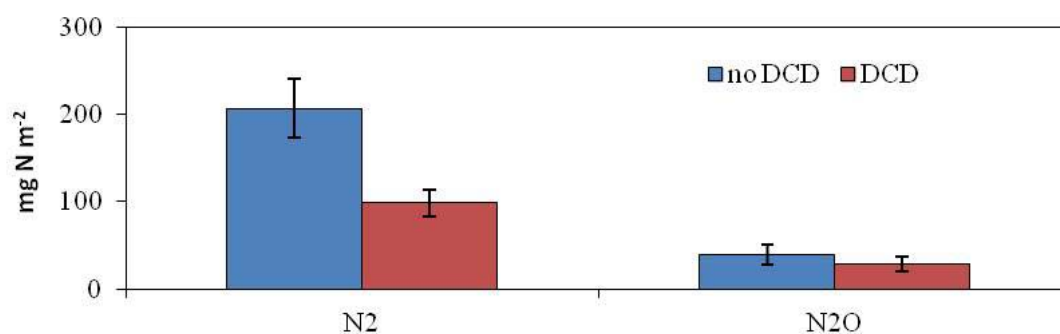
Figure 2. Cumulative \text{N}_2\text{O} and \text{N}_2 emissions, over 20 days after application of cattle slurry, with and without a DCD amendment. The graph shows averages from three grassland sites in Ireland.
