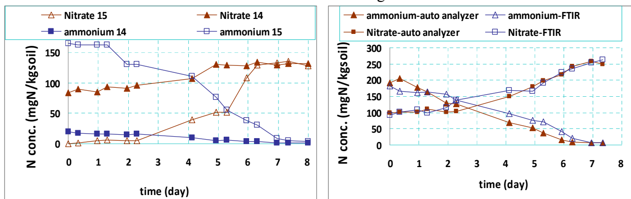
Figure 1. Left: Changes with time of ^{15}\text{N} and ^{14}\text{N} mineral N-species concentrations obtained for incubation of Terra Rosa amended with ^{15}\text{NH}_4 using FTIR spectroscopy; Right: Changes with time of ^{14}\text{N} mineral N-species concentrations obtained for Terra Rosa incubated with ^{14}\text{NH}_4 – FTIR results compared to auto-analyzer measurements.
