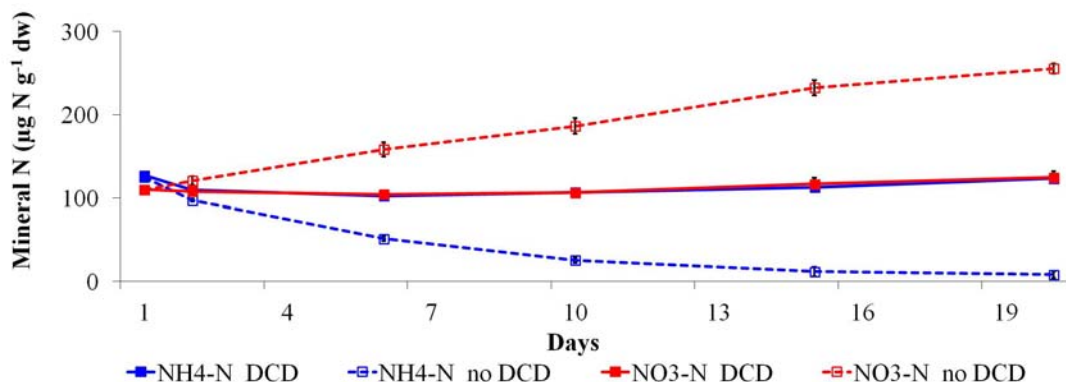
Figure 1. Mean \text{NH}_4^+ and \text{NO}_3^- concentrations in grassland soil, over 20 days after application of cattle slurry, with and without a DCD amendment. The graph shows averages from three sites in Ireland.
