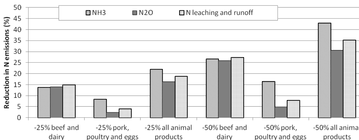
Figure 2. Reduction in EU-27 total \text{NH}_3 and \text{N}_2\text{O} emission and N leaching and runoff for different scenarios with reduced consumption of animal products
