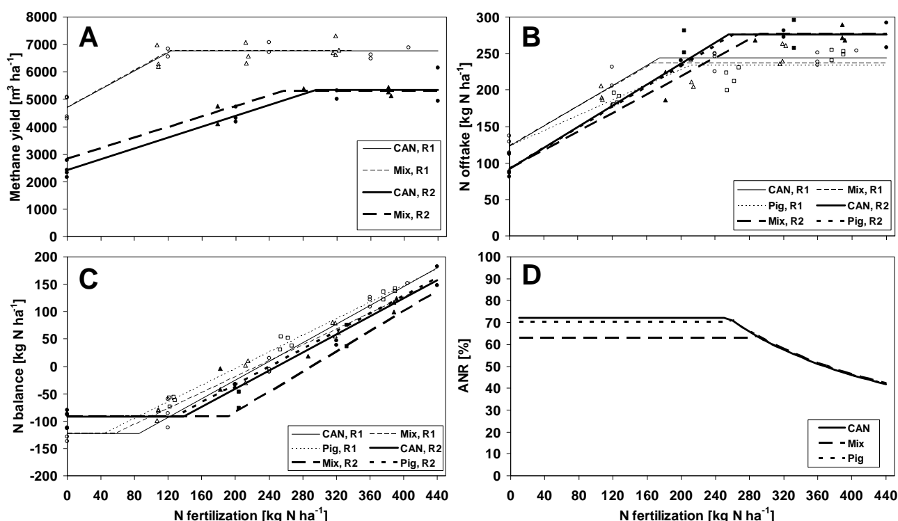
Figure 1. Average annual methane yield ( \text{m}^3 \text{N CH}_4 \text{ ha}^{-1} ) (a), N offtake (b), N balance (c) and apparent N recovery (ANR) (d) of crop rotations R1 (thin lines, open symbols) and R2 (bold lines, closed symbols) fertilized with varying amounts of mineral N (solid lines, circles), biogas residue (broken lines, triangles) and pig slurry (dotted lines, squares).
