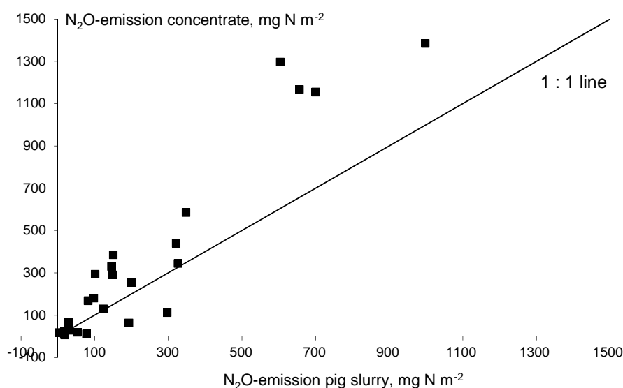
Figure 2. \text{N}_2\text{O} emission from pig slurry against \text{N}_2\text{O} emission from mineral concentrate. Results of all experiments.
