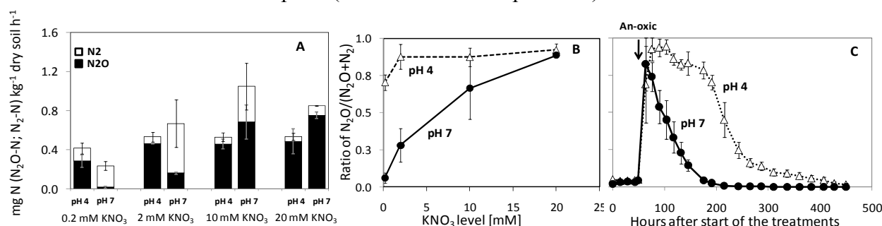
Figure 1. Effect of different \text{KNO}_3 concentrations on A) soil N turnover and emission rates ( \text{mg N kg}^{-1}\text{ dry soil h}^{-1} ), and B) the \text{N}_2\text{O}/(\text{N}_2\text{O}+\text{N}_2) product ratio of denitrification in long-term limed (pH 7) and non-limed control (pH 4) soils in Exp. 1. The course of C) \text{N}_2\text{O}/(\text{N}_2\text{O}+\text{N}_2) product ratios of denitrification at N level of 15 mM \text{KNO}_3 in long-term limed (pH 7) and non-limed control (pH 4) soils in Exp. 2
