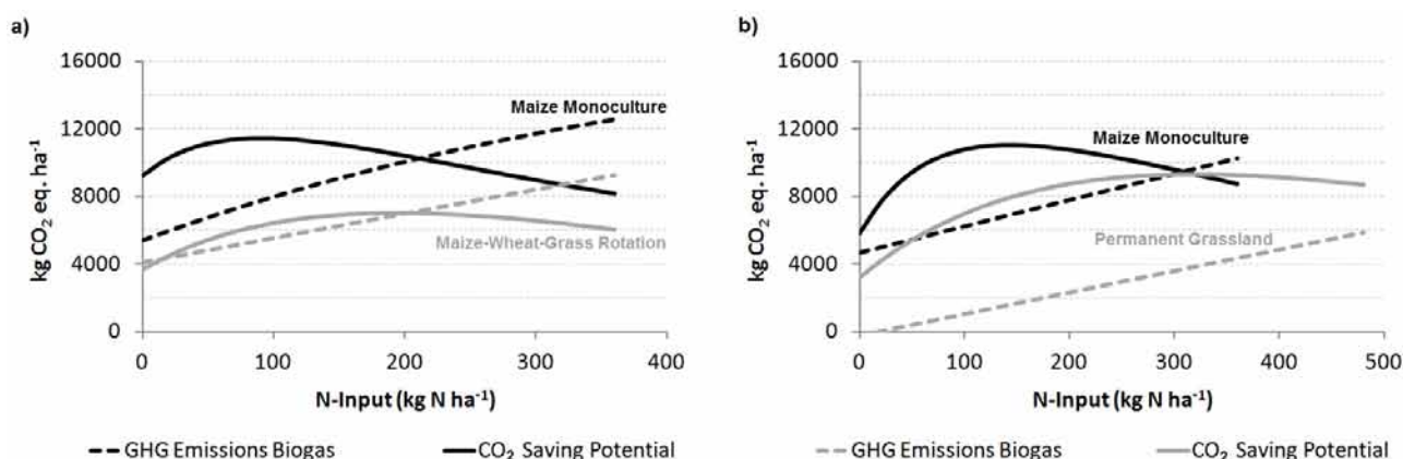
Figure 1. Lines of best fit for relationships between total N-input of CAN ( \text{kg N ha}^{-1} ), \text{CO}_2\text{eq.} emission for the production of energy by biogas and \text{CO}_2\text{eq.} emission saving potential as influenced by cropping system at (a) Hohenschulen and (b) Karkendamm.
